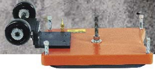
Vacuum Plate with Wheels All purpose vacuum base (A.P.V.) that turns your small anchor base into a vacuum base. Up to 6" diameter core bits accepted. Includes: base, vacuum mount, wheel kit and vacuum gasket.
