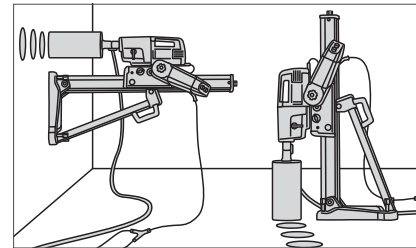
Automatic drilling in all applications.
